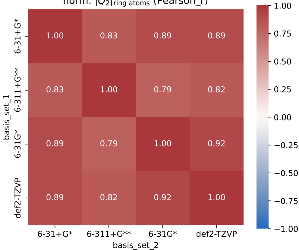
norm: |Q_2|_{\text{ring atoms}} (Pearson_r)
